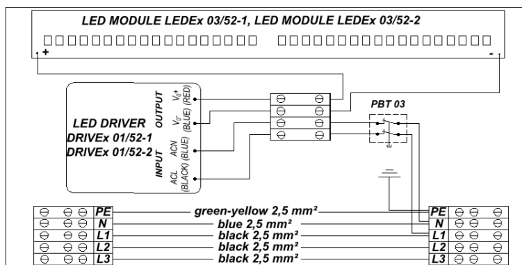
Wiring diagram
